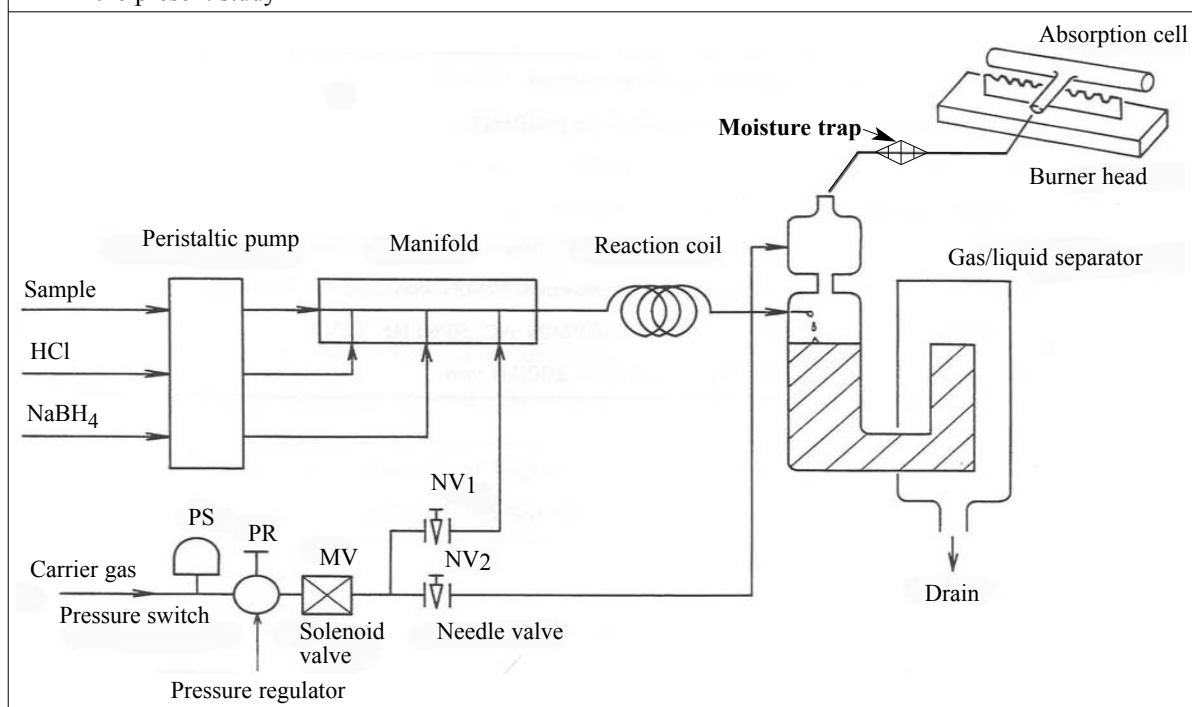
Fig. 1. Modified flow-chart of analysis of arsenic in drinking-water by hydride generation-atomic absorption spectrophotometry (printed with permission from Shimadzu). The moisture trap was developed in the present study
